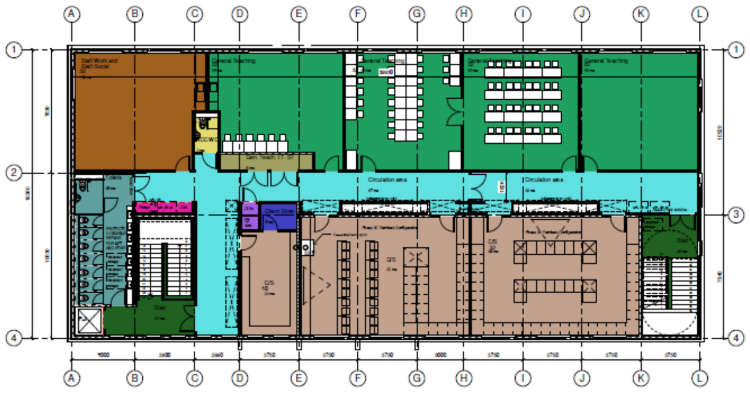
1 Ground Floor Plan 1 : 100
